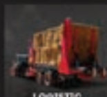
LOGISTIC
